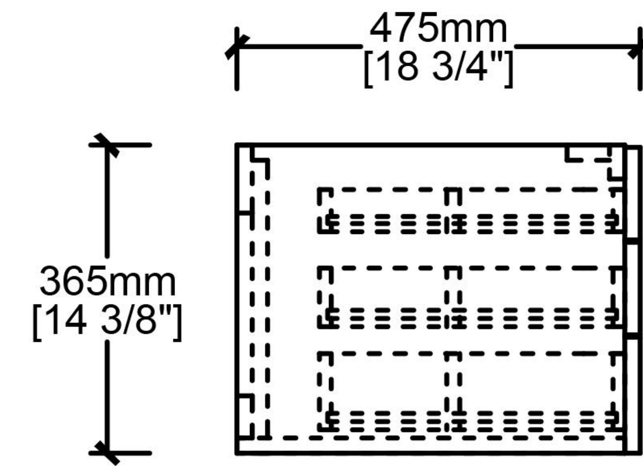
Side View
