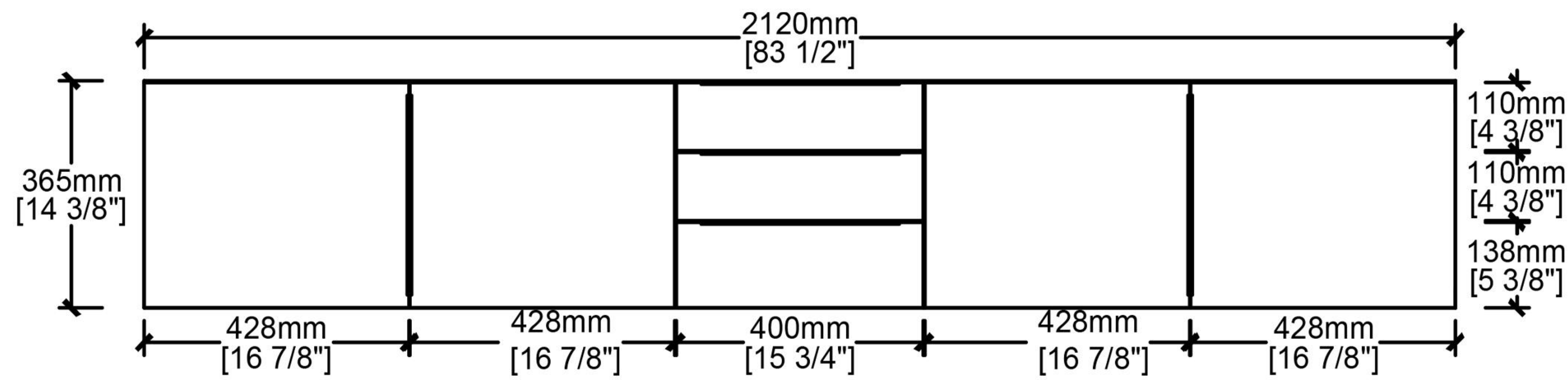
Front view
