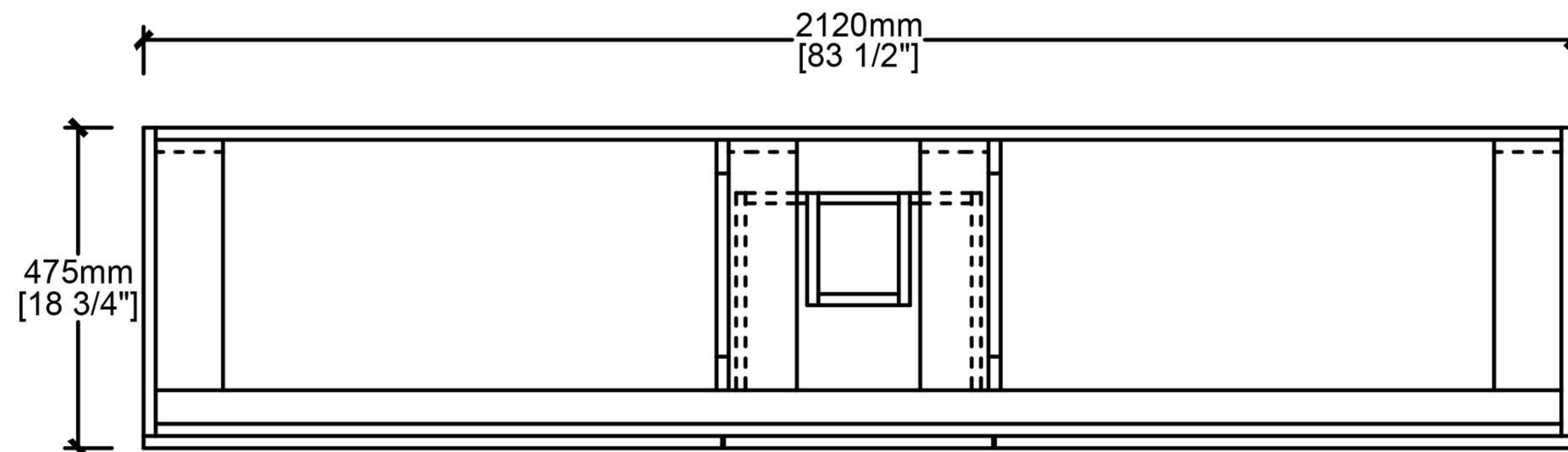
Top View
