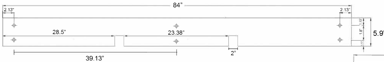
Rear View
