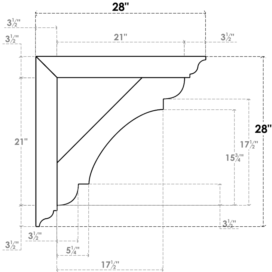
SIDE PROFILE
