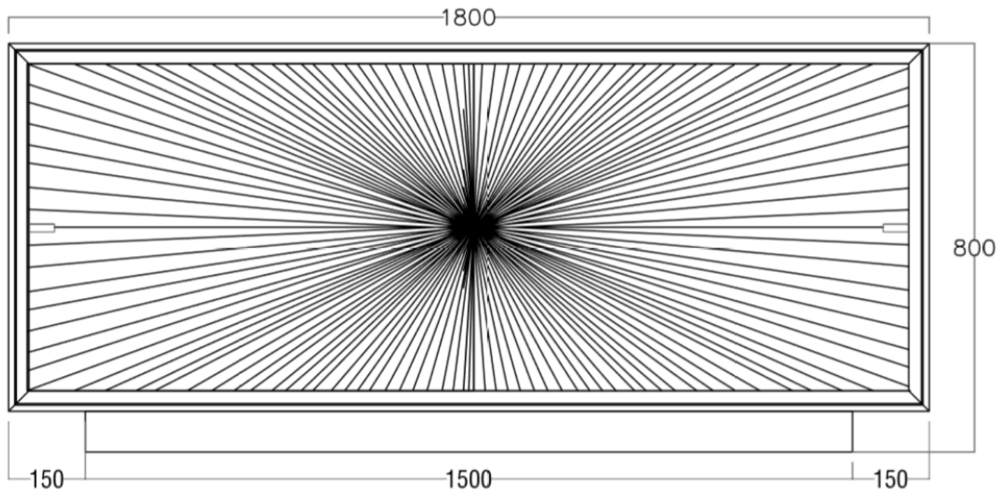
02 FRONT VIEW SCALE 1 : 20
