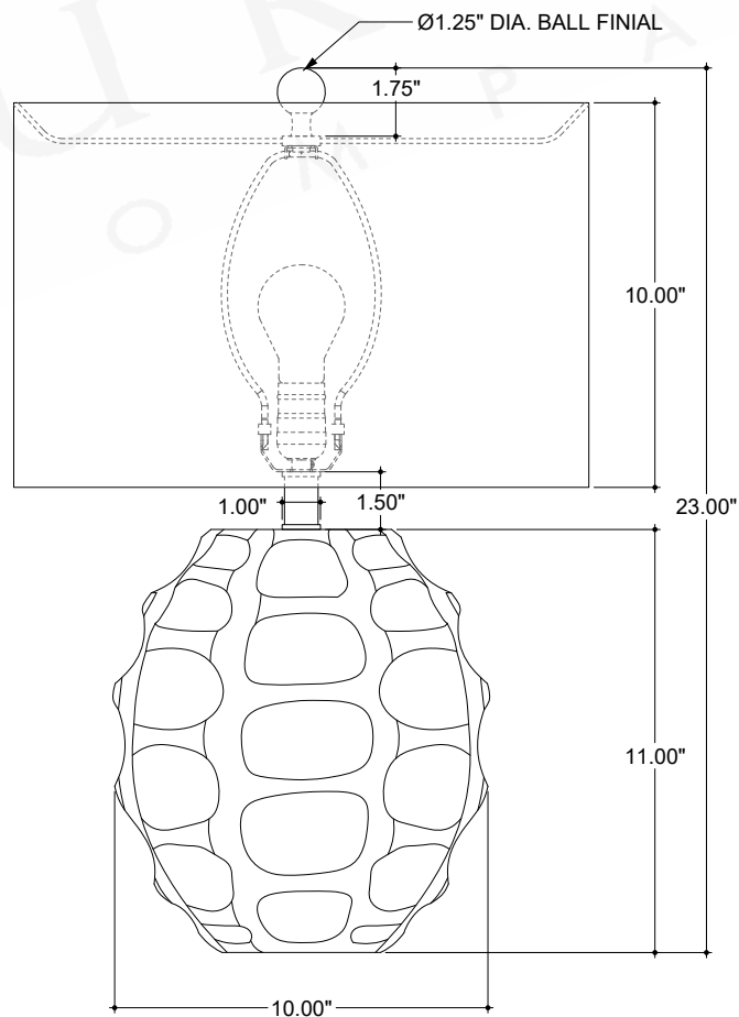
FRONT VIEW
