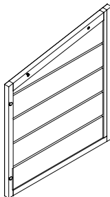
Panel of nesting box(Right) 2PCS
