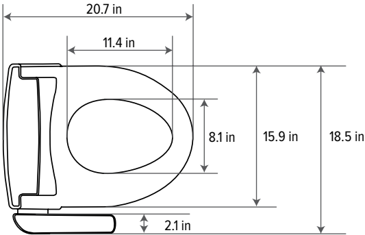
Elongated Top View
