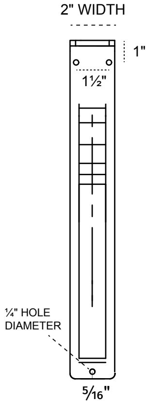
FRONT PROFILE
