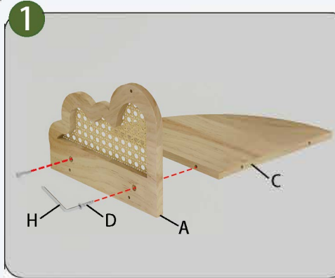
Connecting Part A C.
