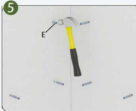
Use a hammer to hammer the expansion tube into the drilling hole.
