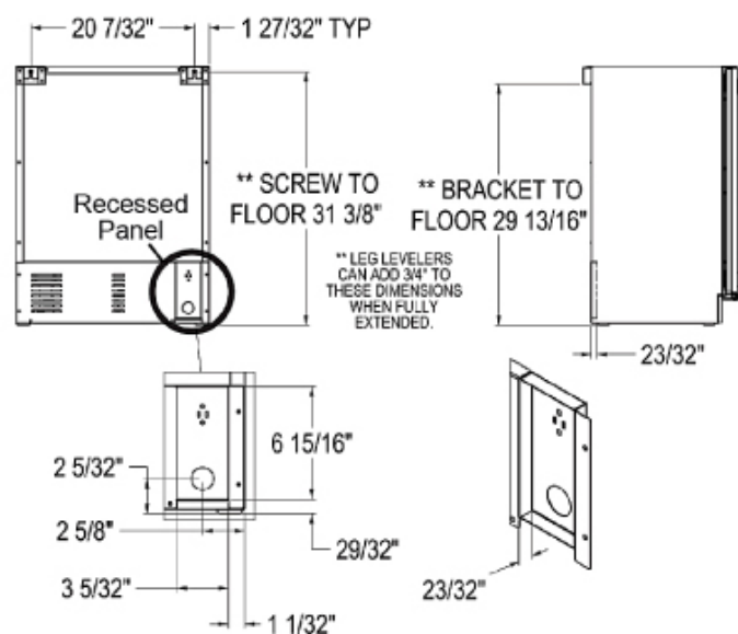
Figure 1. HH (Sottile Model) Electrical Connections
