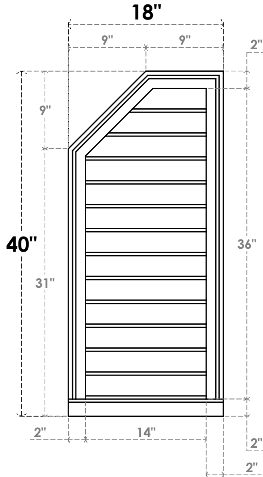
FRONT
