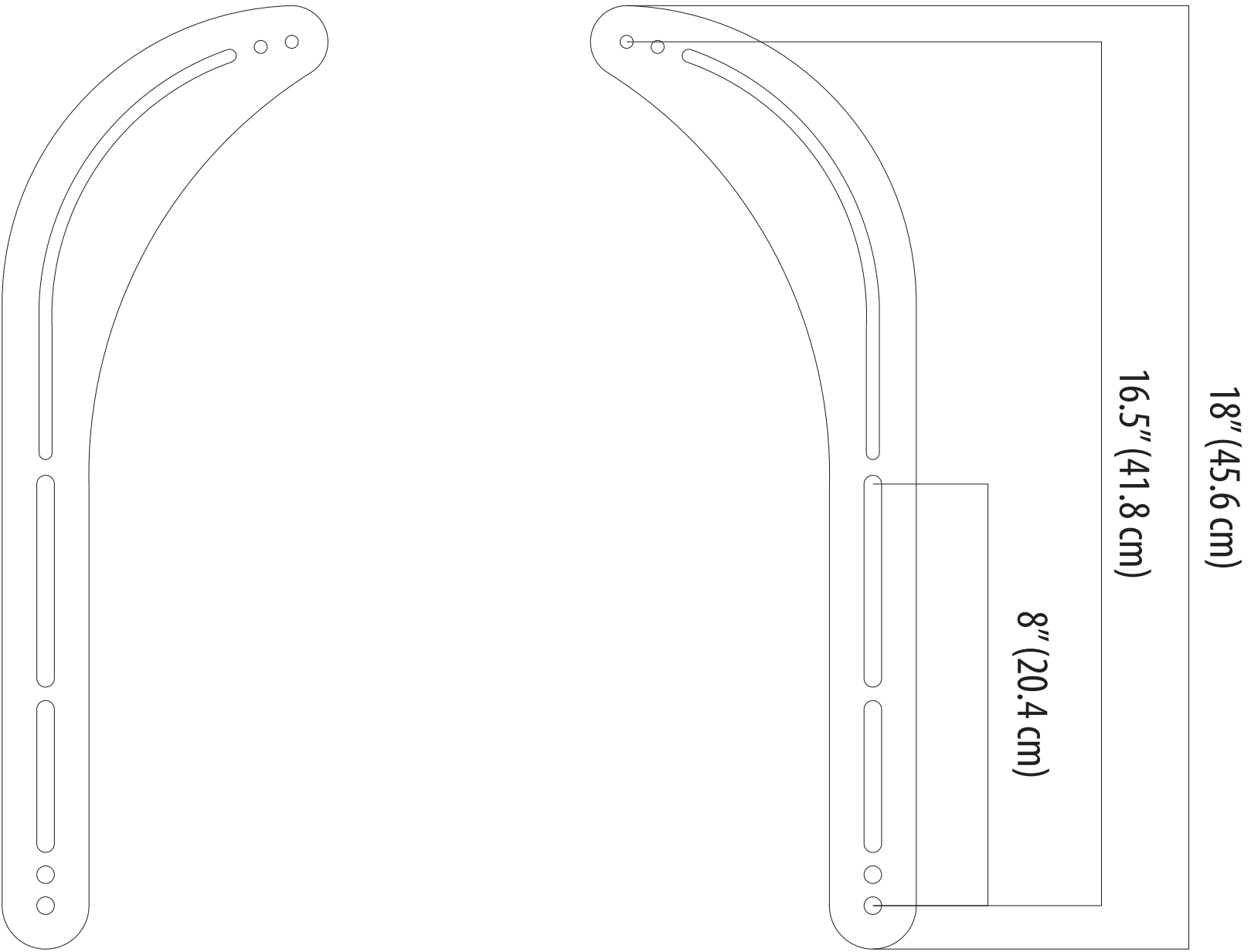
MSB33 / General Dimensions dimmmensions: in (cm)
