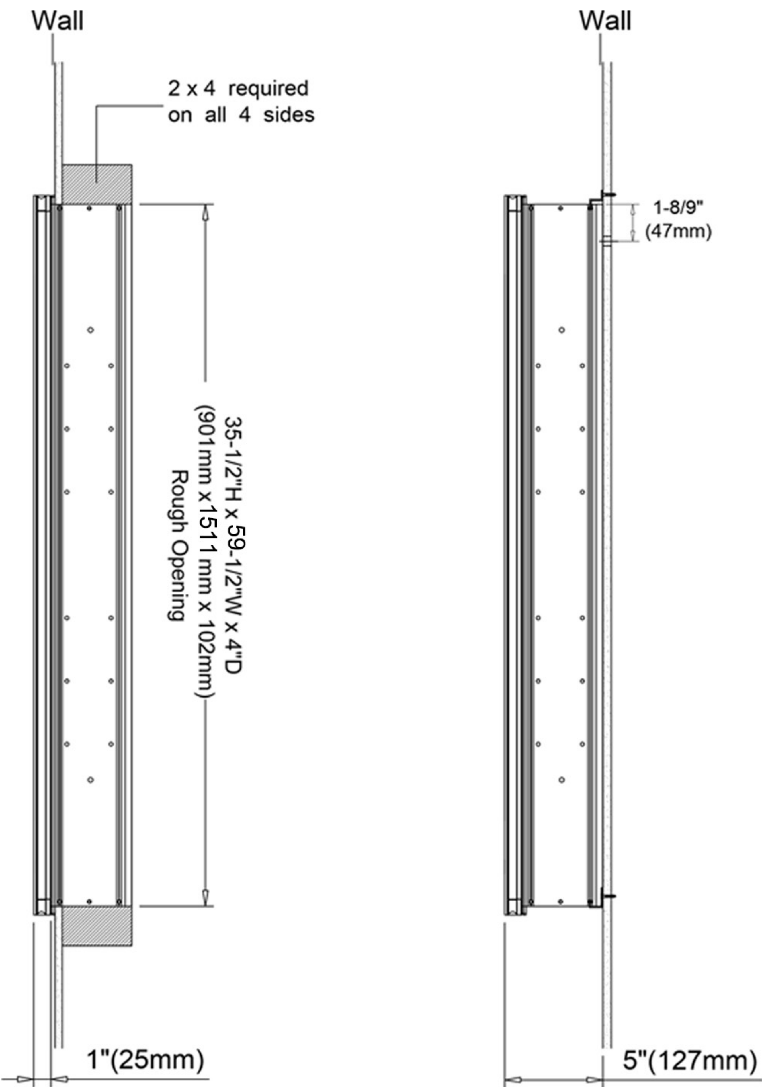
Recessed Mount
