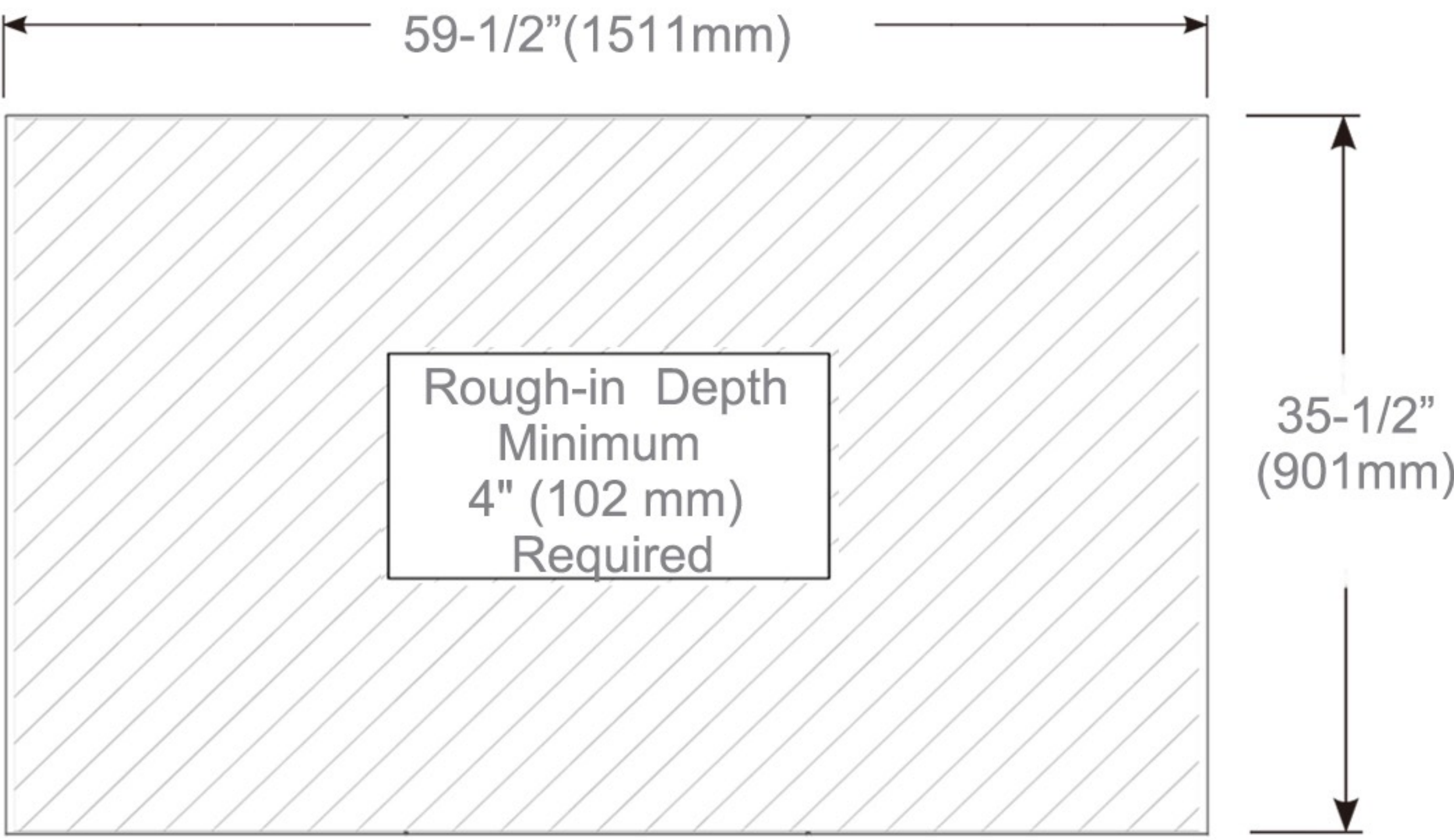
Rough-in Dimensions
