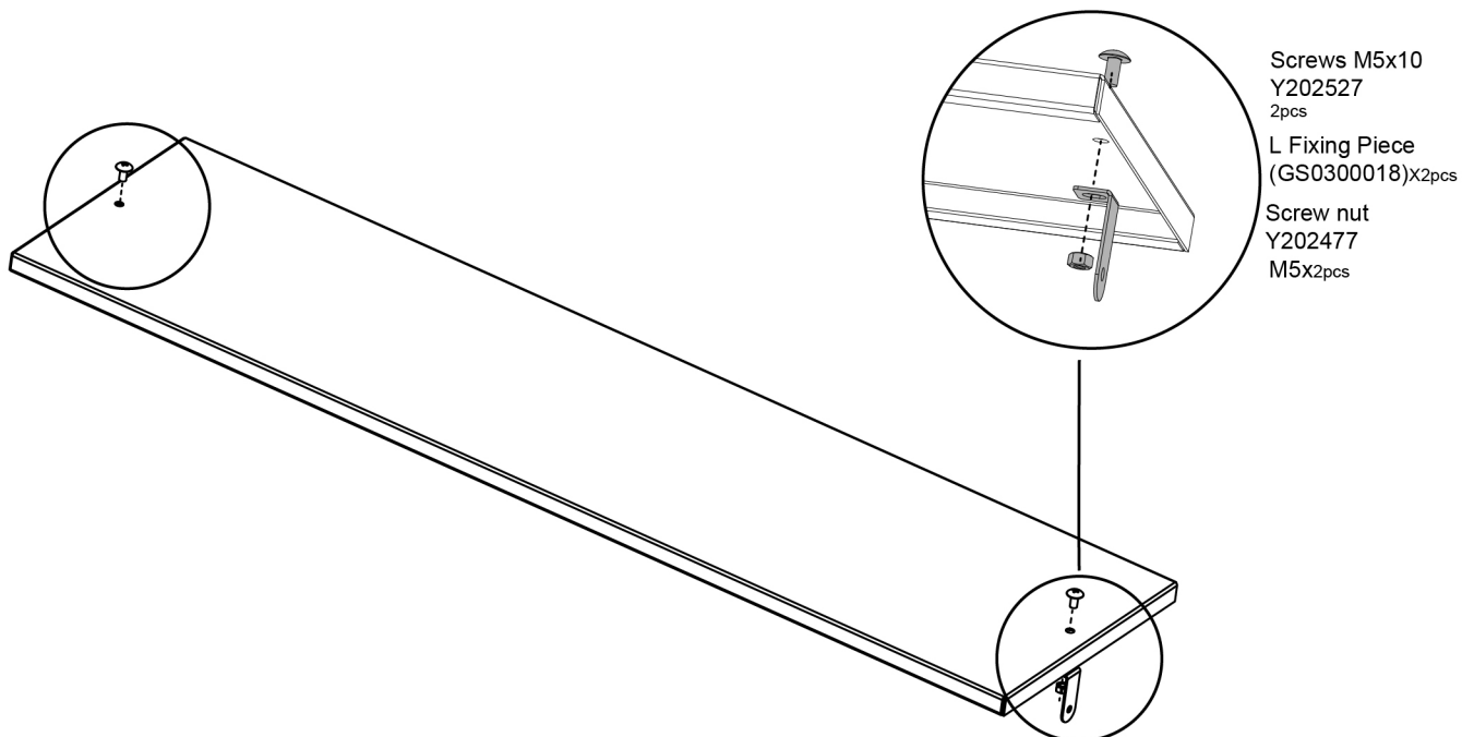
Shelf (GS0300009)X2pcs
