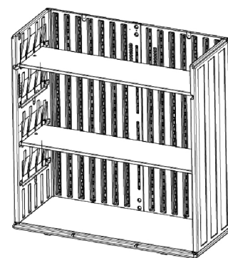
Right back panel GS0300003
