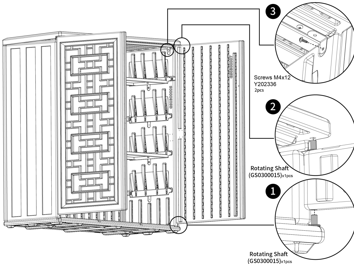
Left Door Panel (GS0300006)X1pcs
