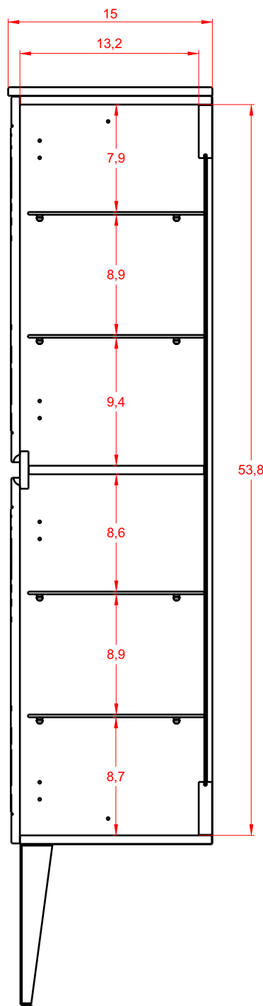
Side view
