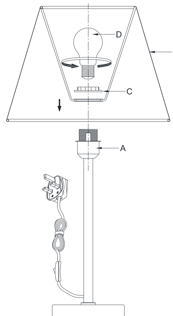
DIAGRAM 1: LAMP ASSEMBLY
