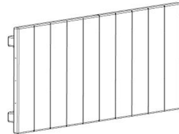
DA1 - DRAWER ASSY - W2A04017 (x1) 1 9/16"x10 3/16"x22 1/16" (40x259x560)
