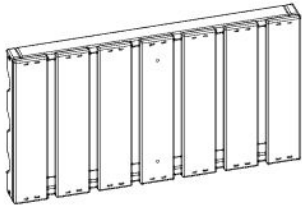
WR1-WINE RACK ASSY - W2A04016 (x2) 1 13/16"x11 1/8"x19 15/16" (46x283x506)
