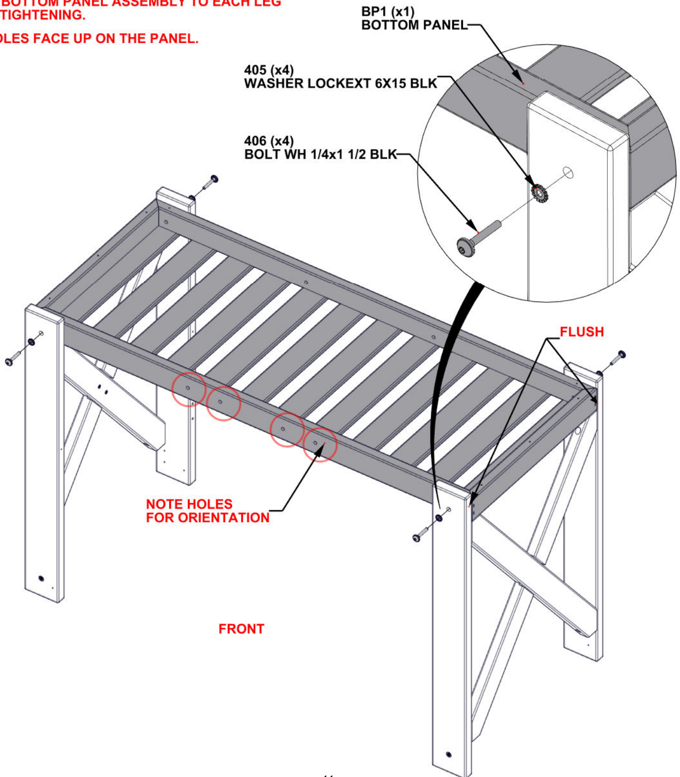
BP1 - BOTTOM PANEL - W2A04015 (x1) 2 3/8"x18"x44 5/16" (60x458x1125)
