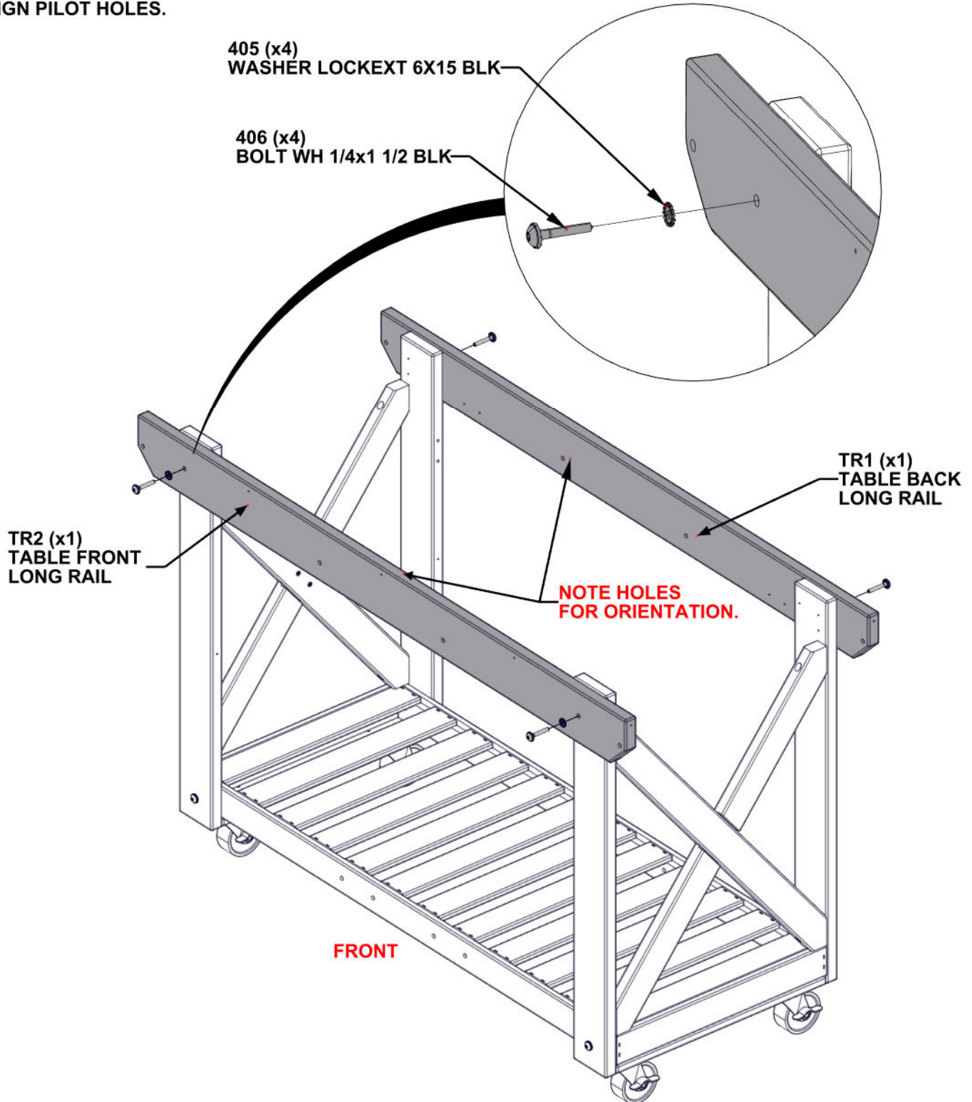
TR2 - TABLE FRONT LONG RAIL - W4L18895 (x1) 15/16"x4"x50 11/16" (24x102x1287)
