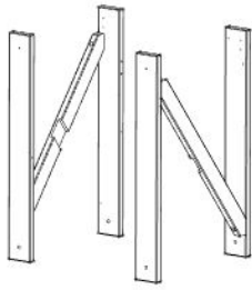
LEG AND CROSS BRACE ASSEMBLY - STEP - 1A
