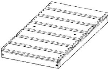
WINE RACK ASSEMBLY - STEP 27A
