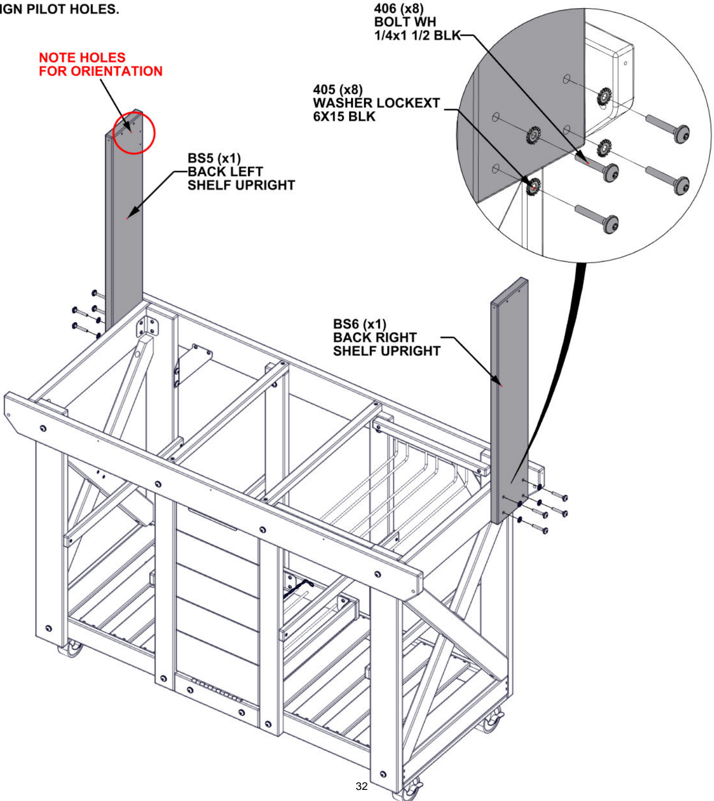
BS5 - BACK LEFT SHELF UPRIGHT - W4L18905 (x1) 15/16"x5 1/4"x27 11/16" (24x134x703)
