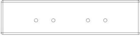
DB2 - DRAWER BACK BOARD - W4L20012 (x1) 5/8"x2 3/8"x9 1/2" (16x60x241)
