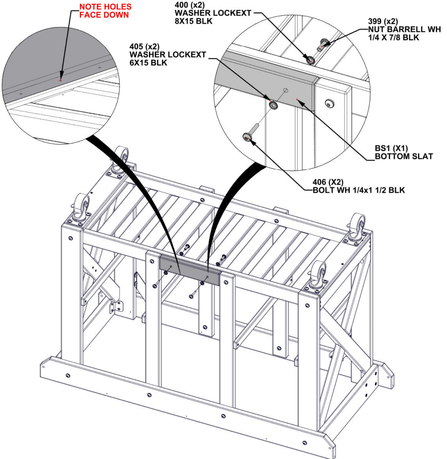
BS1 - BOTTOM SLAT - W4L18901 (x1) 15/16"x2 3/8"x10 3/8" (24x60x263)
