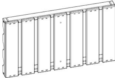
WR1 - WINE RACK ASSY - W2A04016 (x2) 1 13/16"x11 1/8"x19 15/16" (46x283x506)
