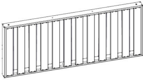
BP1 - BOTTOM PANEL - W2A04015 (x1) 2 3/8"x18"x44 5/16" (60x458x1125)
