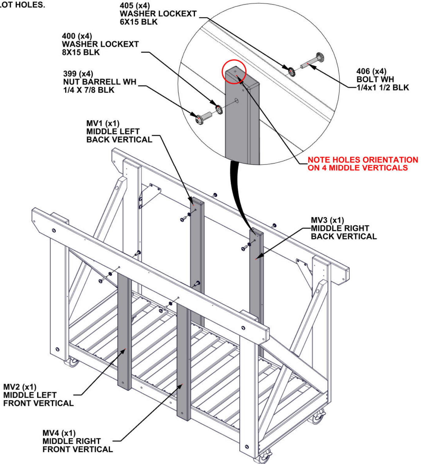
MV2 - MIDDLE LEFT FRONT VERTICAL - W4L18897 (x1) 15/16"x2 3/8"x27 15/16" (24x60x709)
