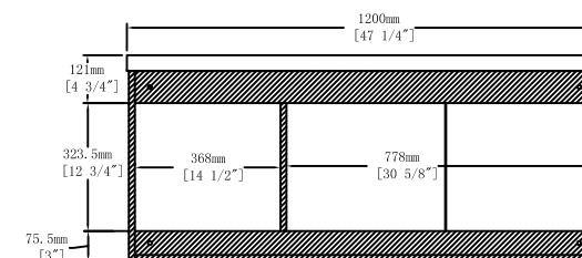
Back View
