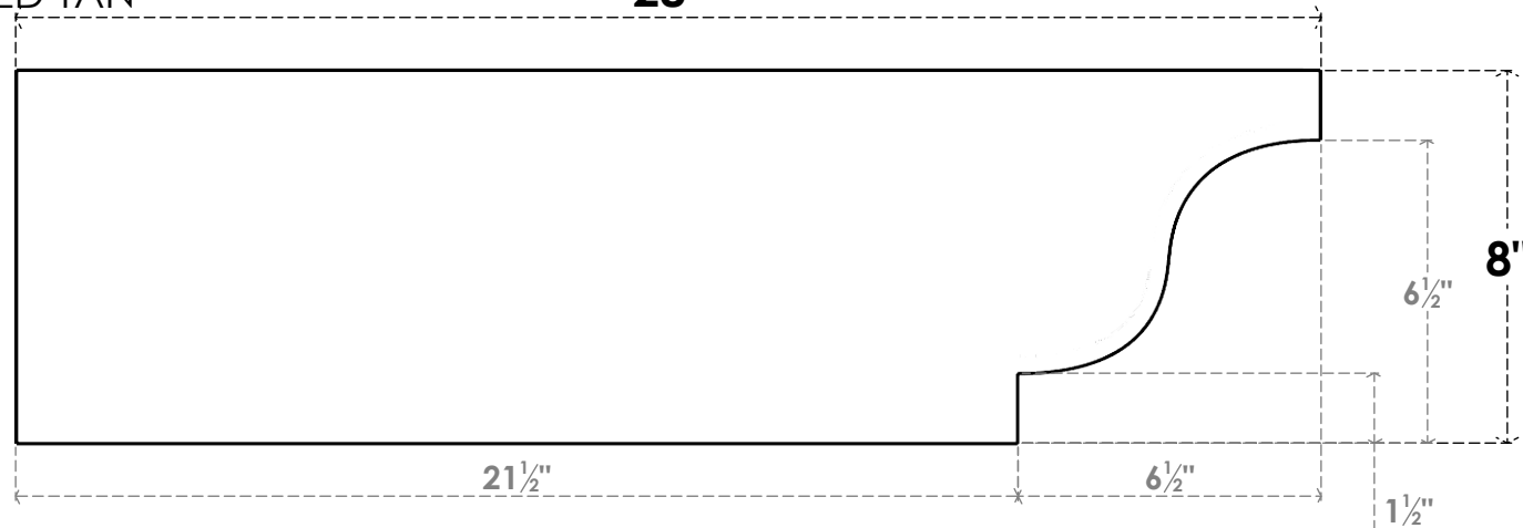
SIDE PROFILE
