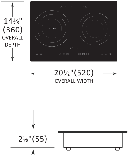
Overall Dimensions
