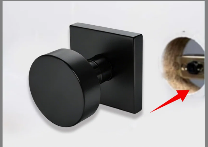
2.CONNECT THE INTERIOR AND EXTERIOR LEVER THROUGHT THE LATCH
