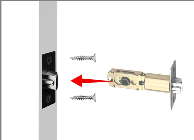
1.SCREW IN THE ADJUSTABLE LATCH
