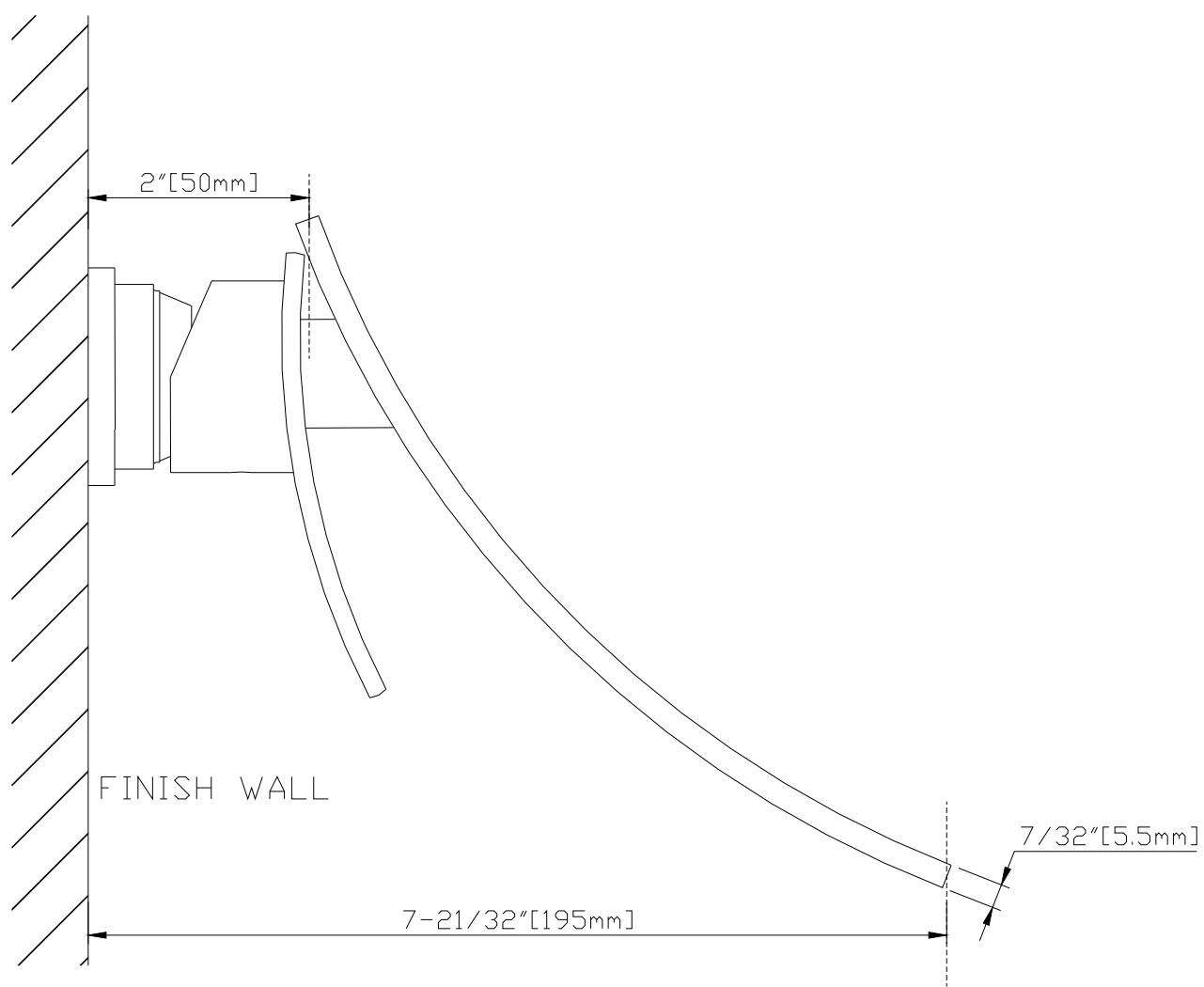
SIDE VIEW OF FAUCET
