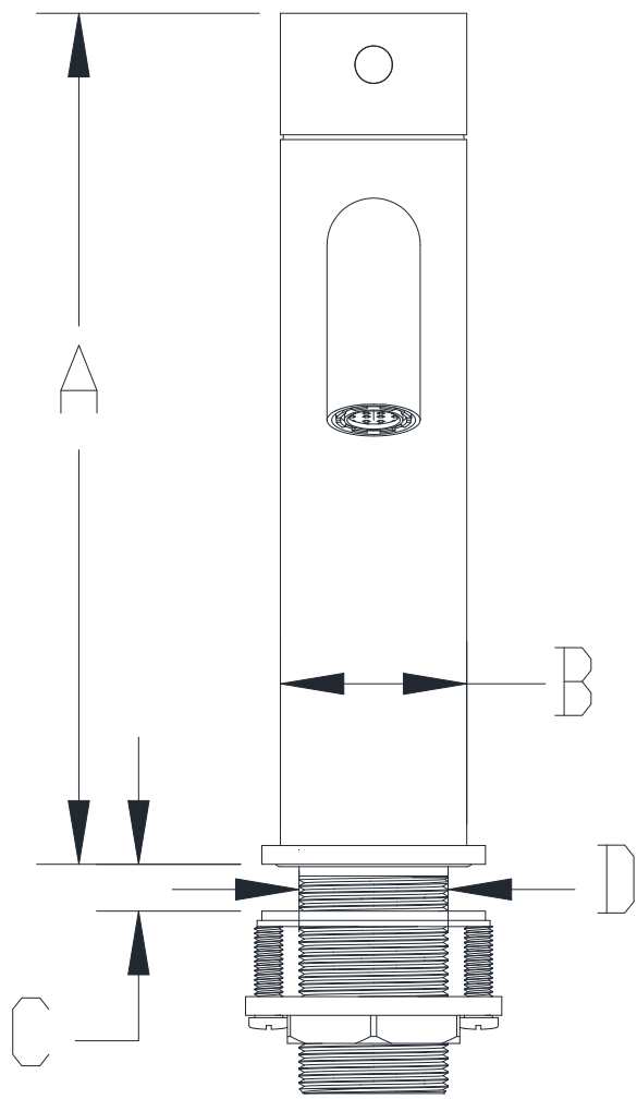
FRONT VIEW OF FAUCET
