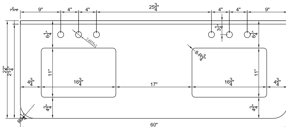
TOP VIEW OF VANITY CABINET
