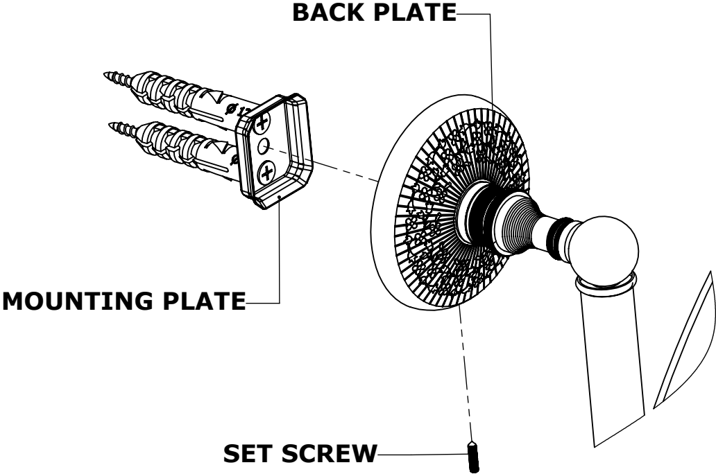
DETAIL N
