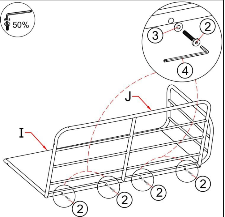
Step 10: Connect Seat Right Frame (I) & Double Back Frame (J), tighten Bolt (2), Flat Washer (3) with Allen Key (4).
