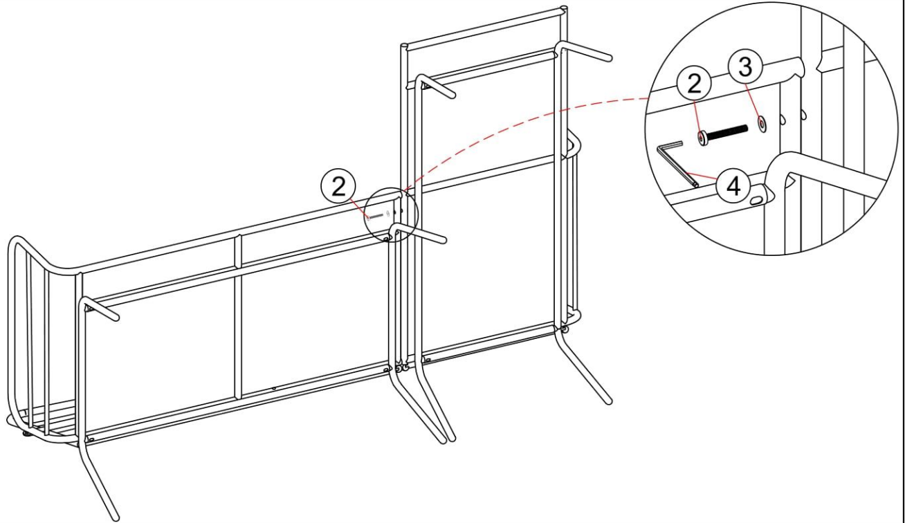
Step 16: Connect The Part from Step 15, tighten Bolt (2), Flat Washer (3) with Allen Key (4).
