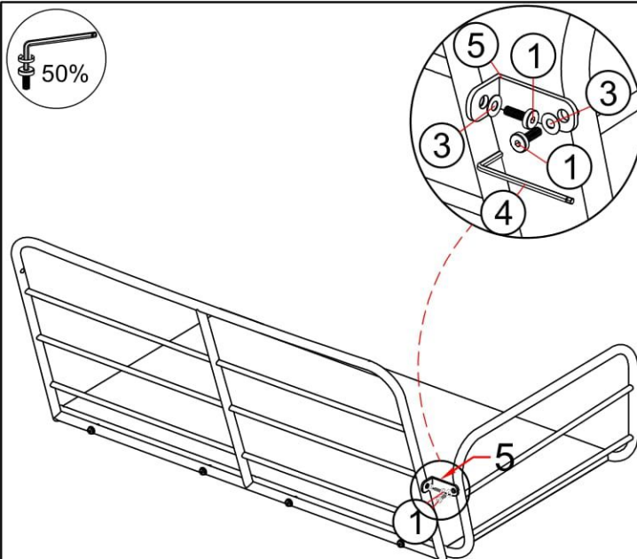
Step 9: Put the Left Bench upright and make sure all legs are level, then firmly tighten bolts with Allen Key (4).
