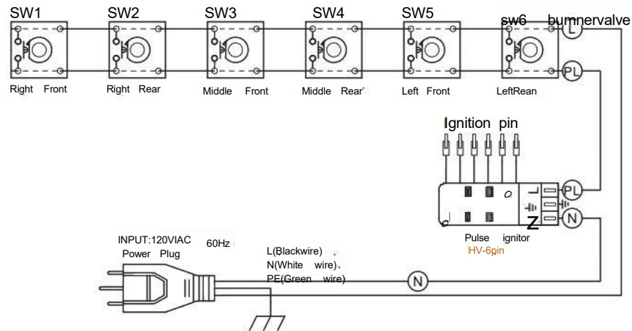
WFCT8536 Circuit Diagram
