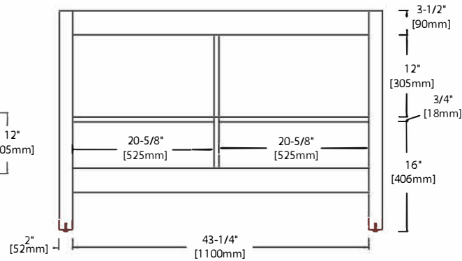
BACK VIEW
