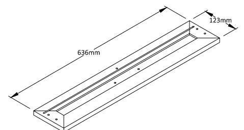
DRAWER FRONT Qty:1
