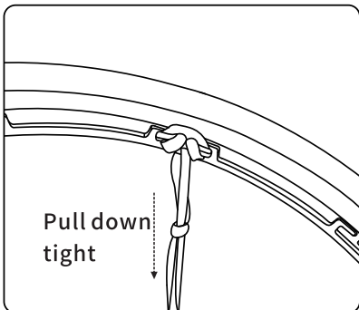
5 Tighten the basketball net downwards so that the ropes passing through the hanging holes form a double knot.
