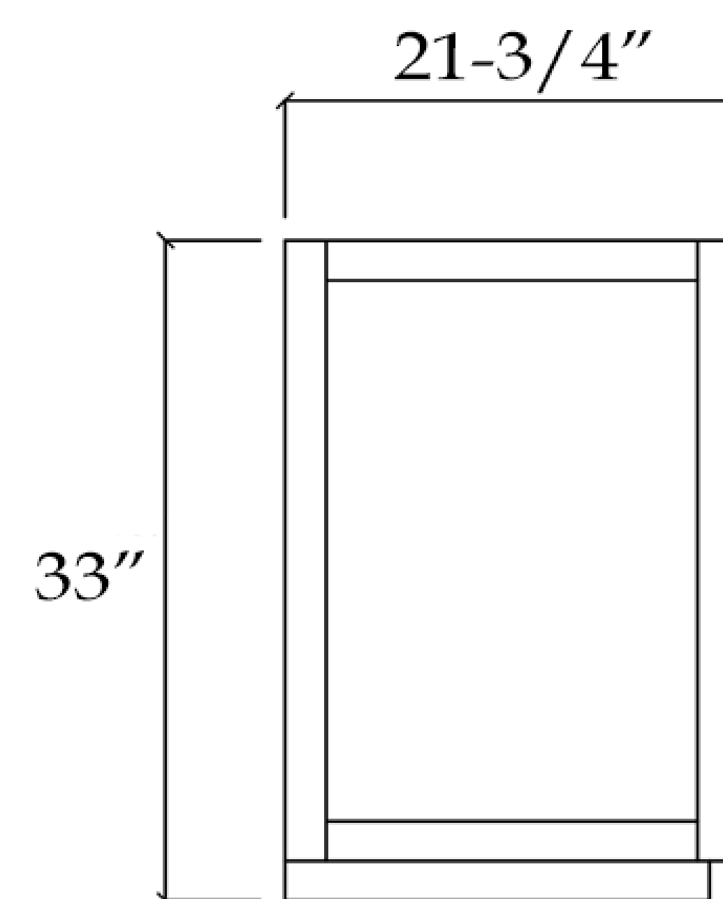
SIDE VIEW
