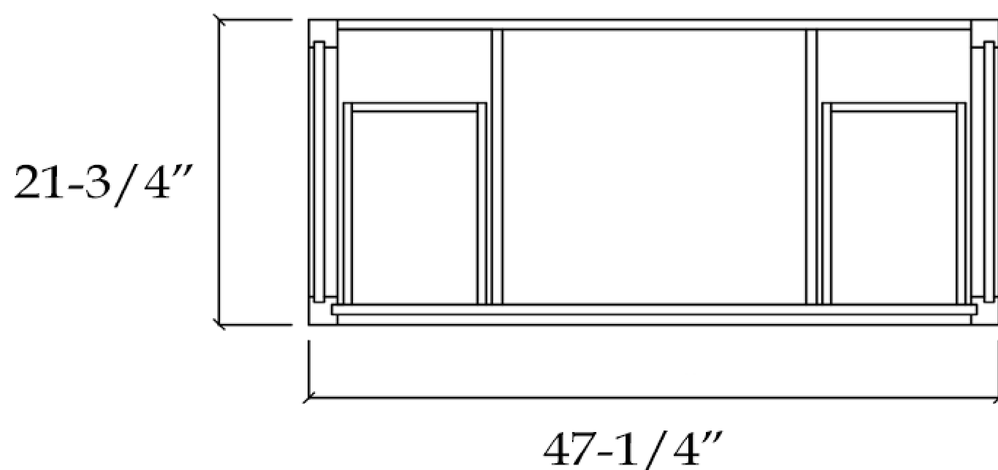
TOP VIEW
