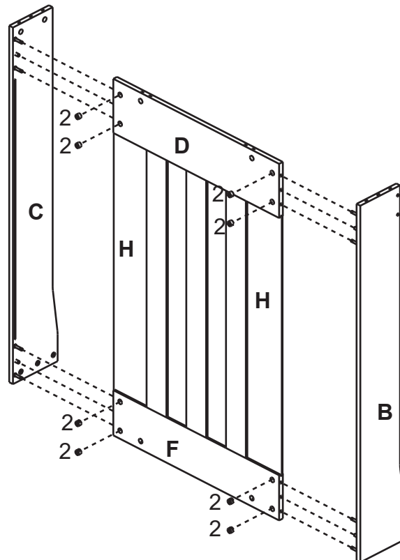
Cam Lock Fastening System
