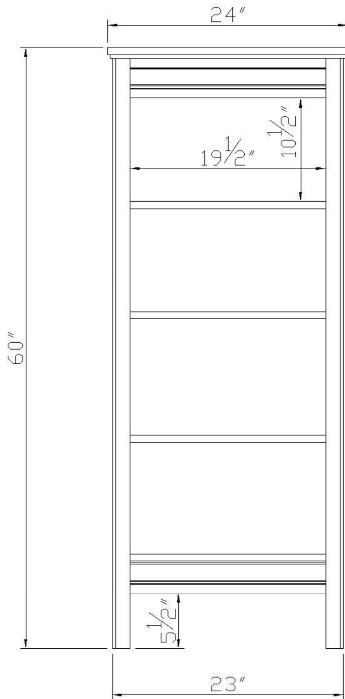
FRONT VIEW
