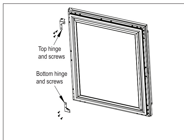
Figure 14. Door Hinges
