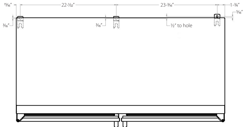
Figure 3. 48" Anti-tip Kit
