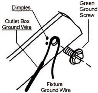
Grounding Detail
