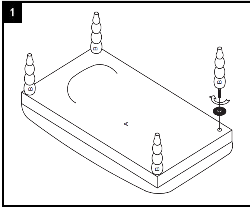
Step 1 Attach four legs(B) to seat (A), using Plastic anti-skid pad (1), and tighten legs
