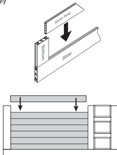
Figure 8 Starter Panel
