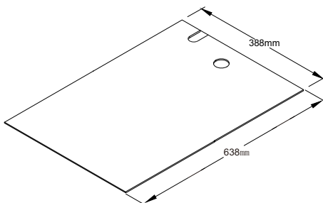
BACK PANEL Qty: 2
