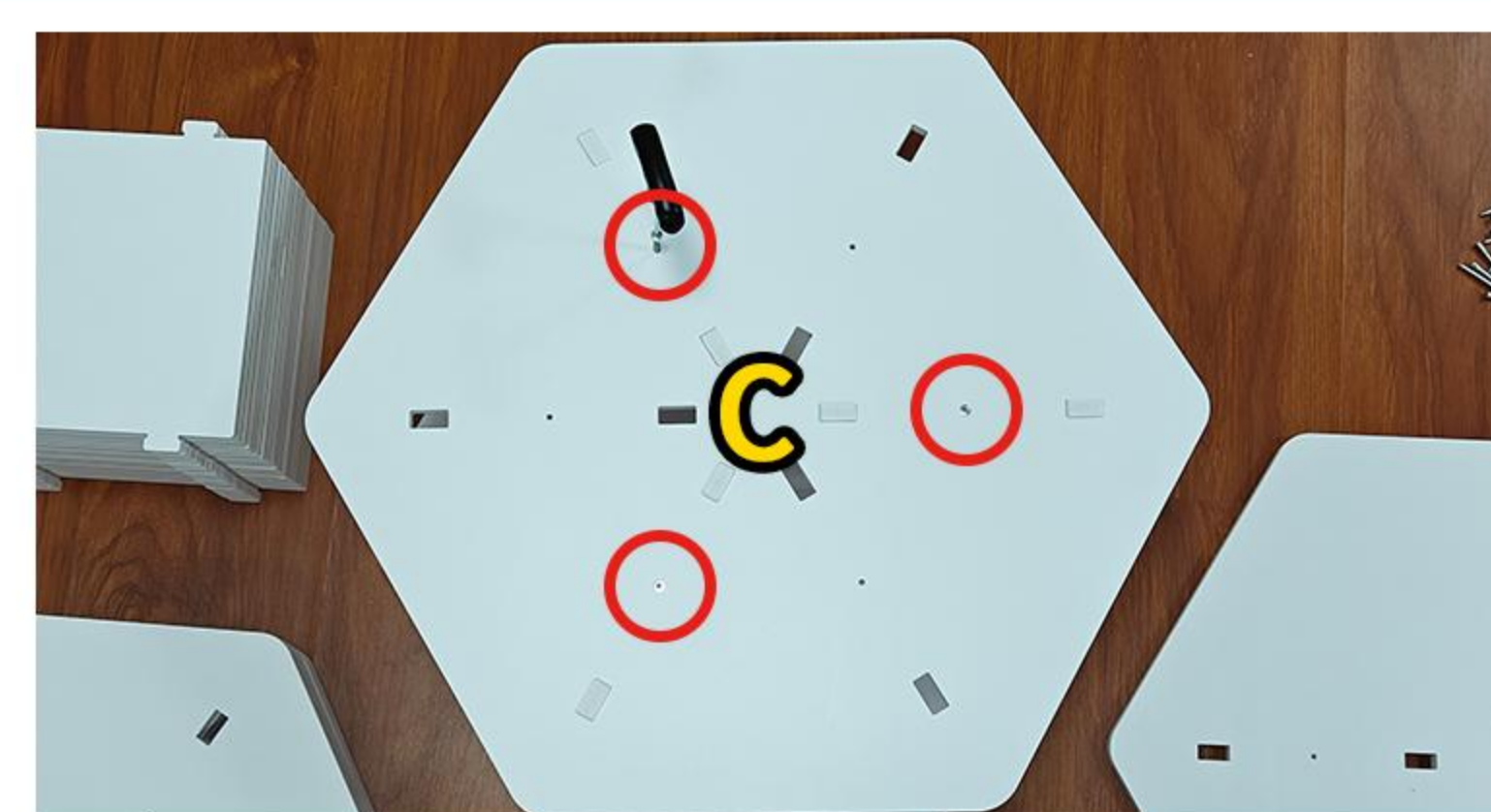
3. TIGHTEN THREE SCREWS
