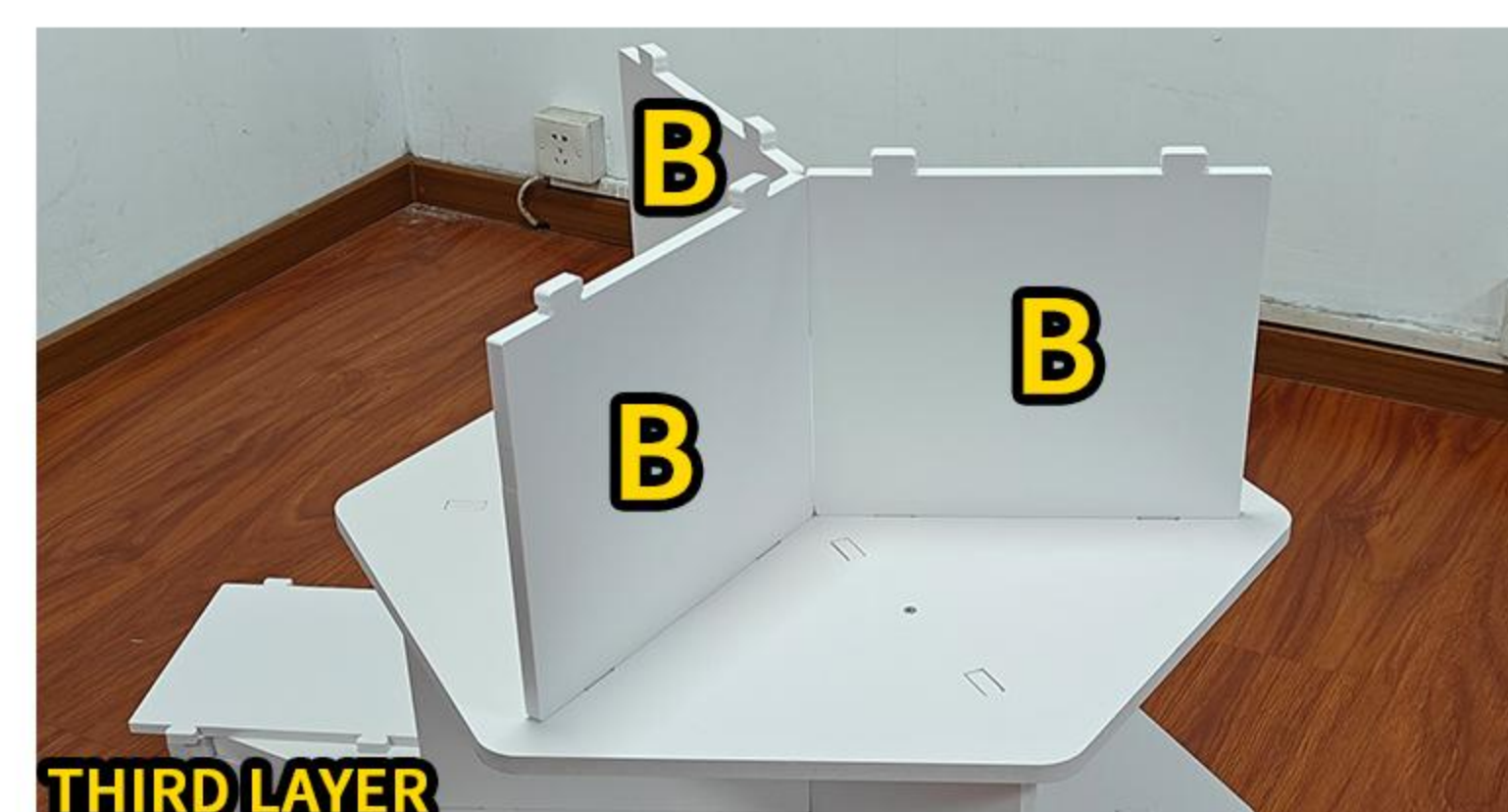
9. INSTALL THREE B-BOARDS
