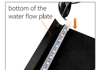
3. Clip the light to the waterfall light strip slot.
