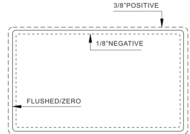
Flushed/Zero Reveal
