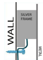
Wall mount detail
