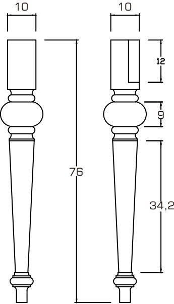
LEG DETAIL
