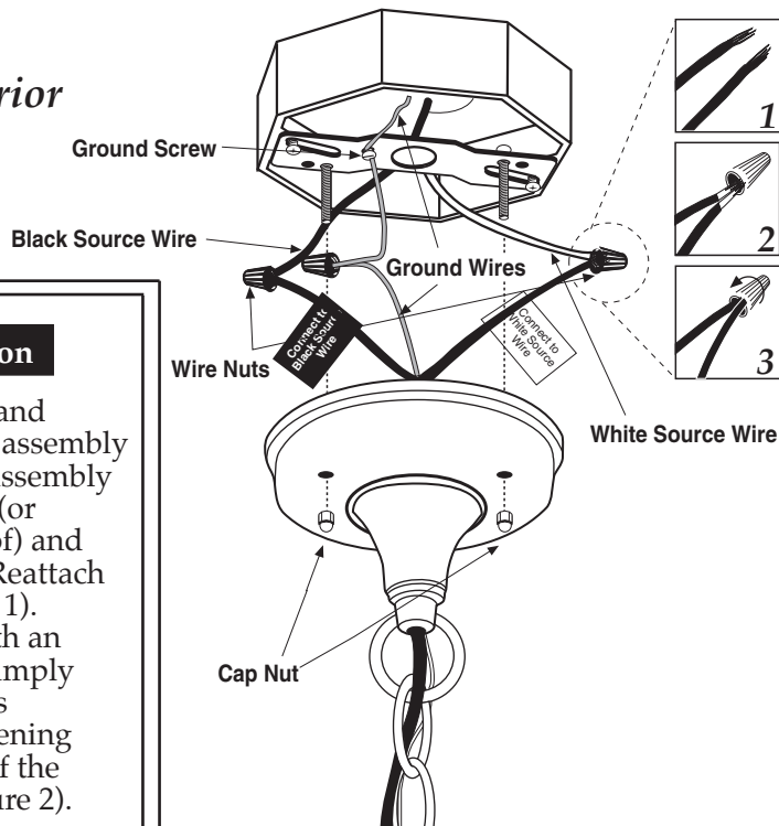
Figure 1 Two Screw Assembly
