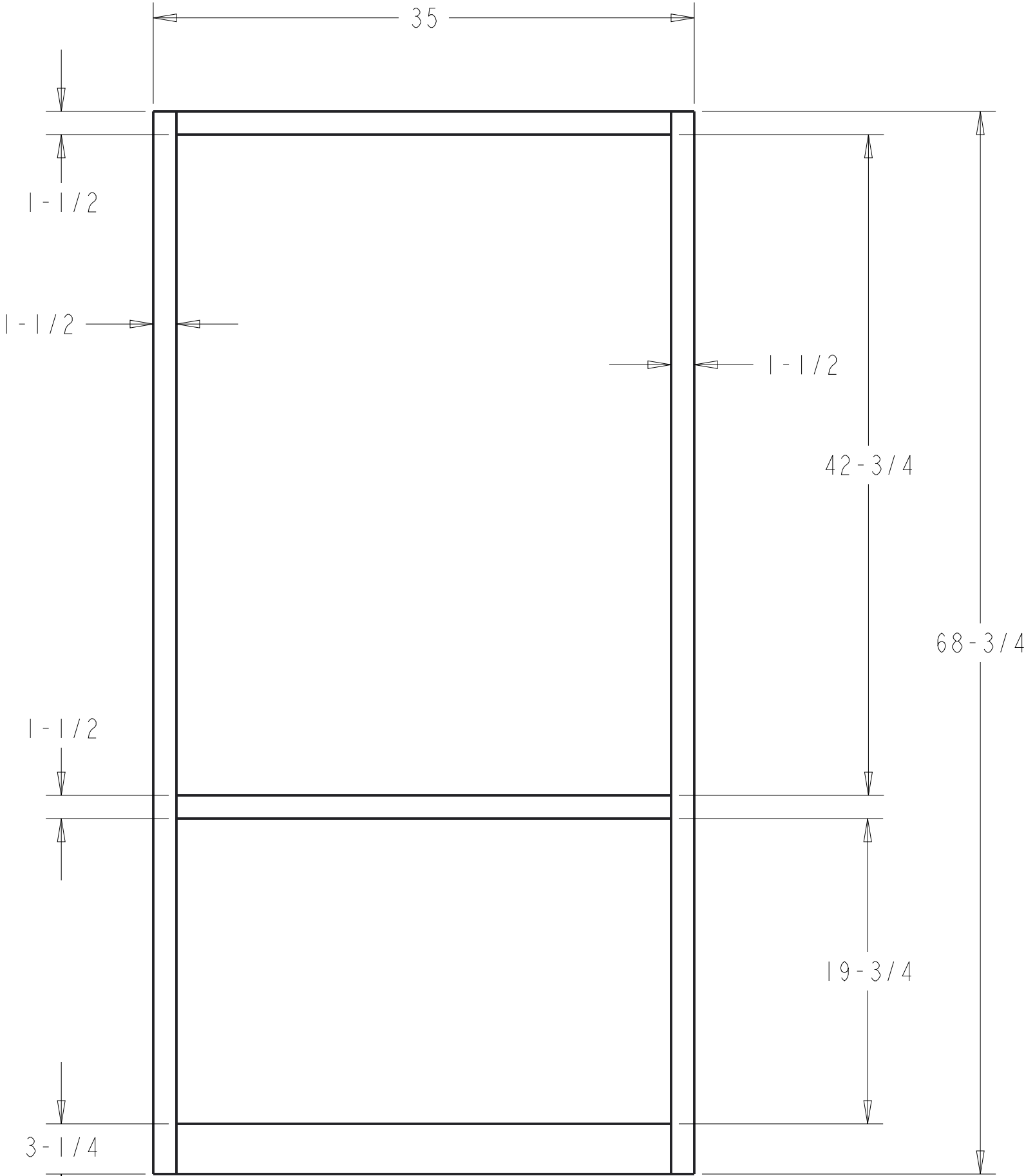
FACE FRAME DETAILS
