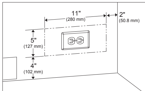
Electrical Location
