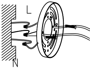
Option A - Junction Box mount
