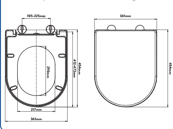
D-Shape Toilet Seat Dimension Drawing.
