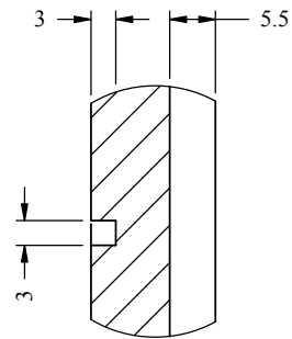
DETAIL BD SCALE 1 : 1
