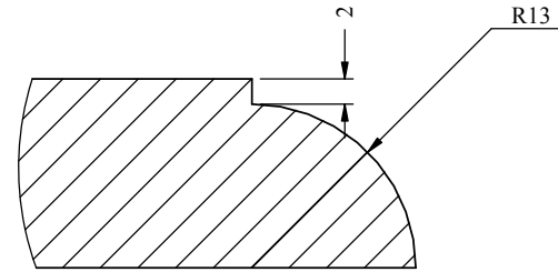
DETAIL BK SCALE 3 : 2
