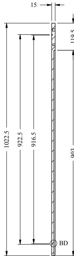
SECTION BC-BC SCALE 1 : 10
