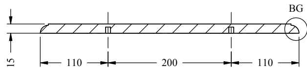
SECTION BF-BF SCALE 1 : 6
