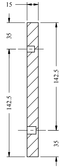
SECTION BM-BM SCALE 1 : 3
