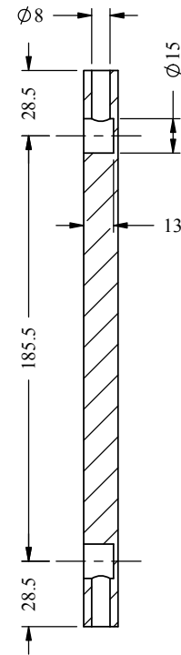
SECTION BN-BN SCALE 1 : 3
