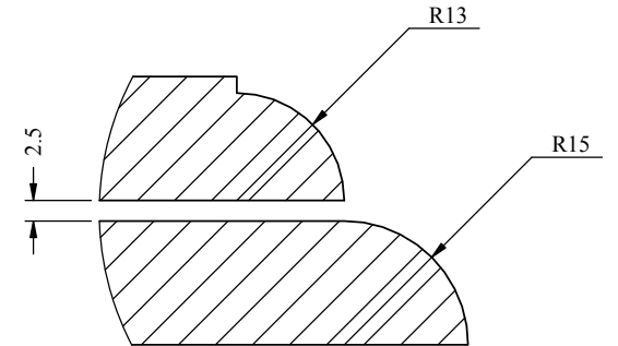
DETAIL BP SCALE 1 : 1
