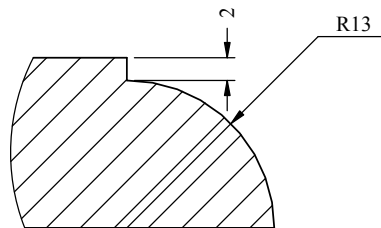
DETAIL BG SCALE 3 : 2
