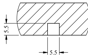
DETAIL BE SCALE 1 : 1
