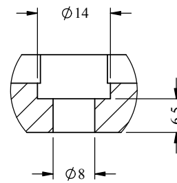
DETAIL BR SCALE 1 : 1
