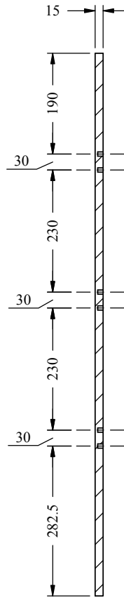
SECTION AY-AY SCALE 1 : 10
