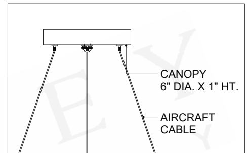
CANOPY DETAIL
