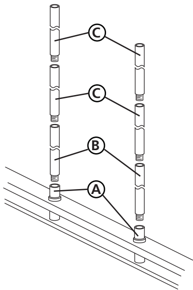
Drawing 1 – Assembly
